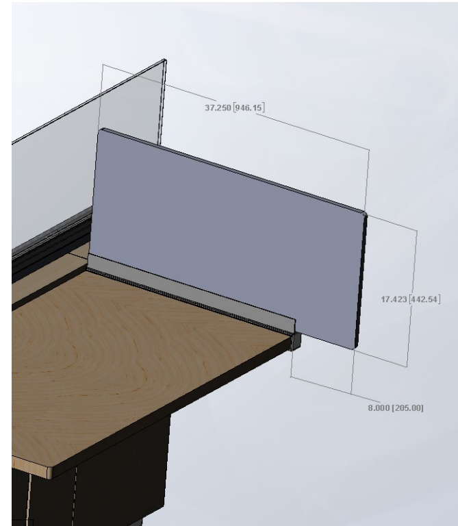
18" HIGH X 37.25" DEPTH SCREEN – EXTENDS 8" PAST USER EDGE
